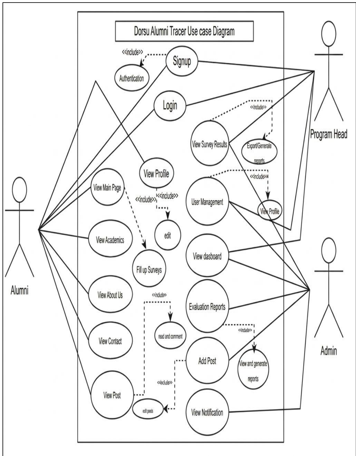
Figure 15. Use Case Diagram (Narrative)
