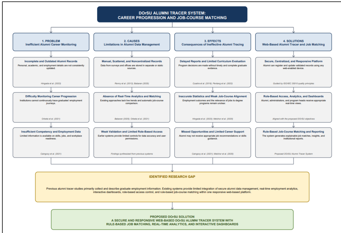
Figure 2. Literature Map
