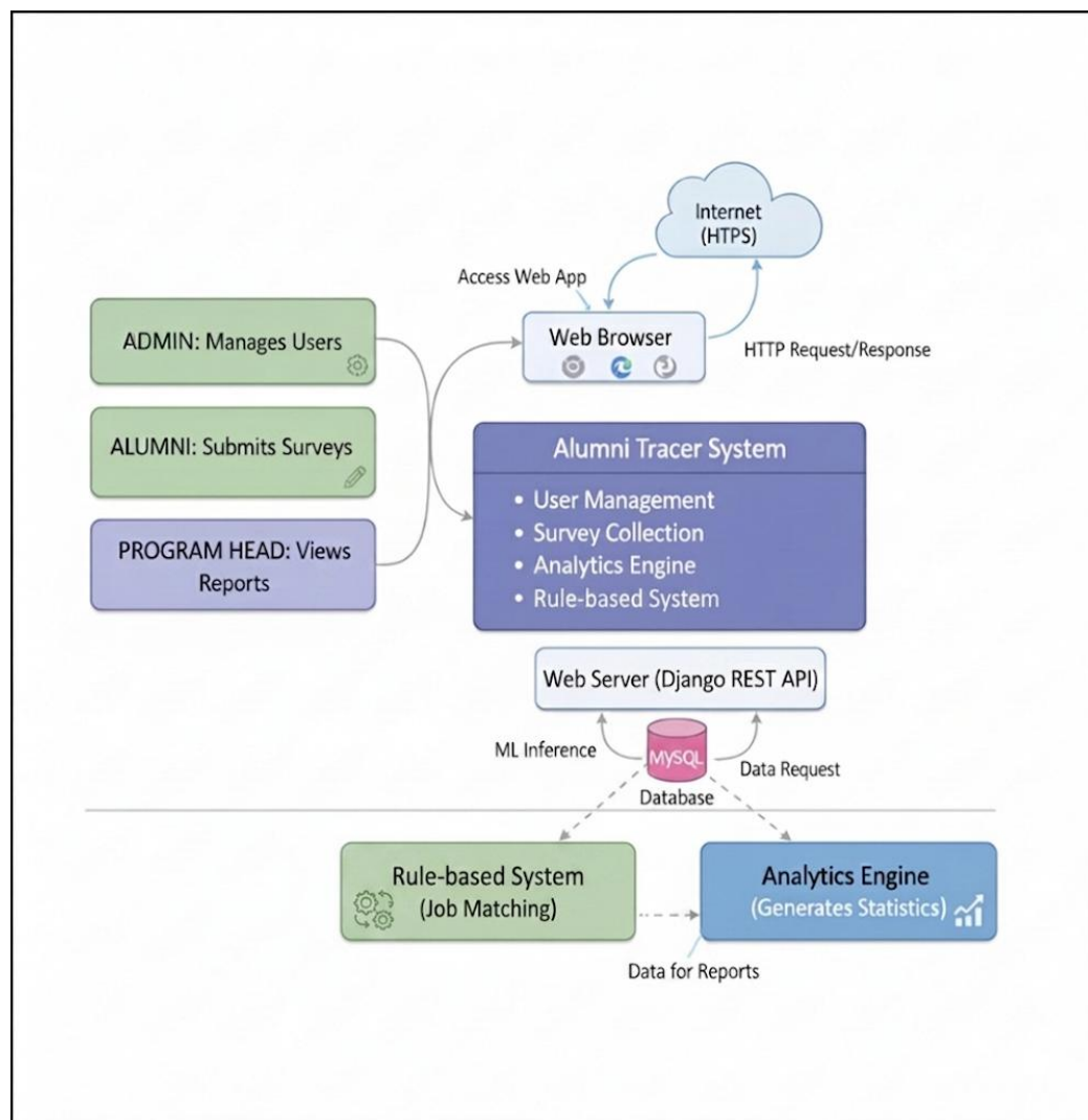
Figure 11. System Architecture
